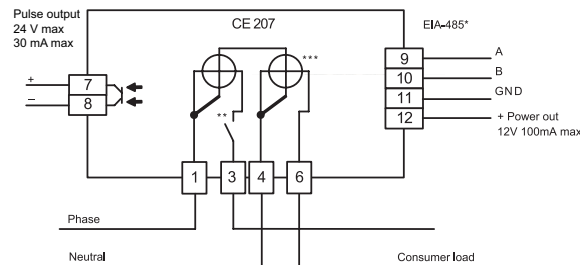
Fig. 1. Meter connection diagram
